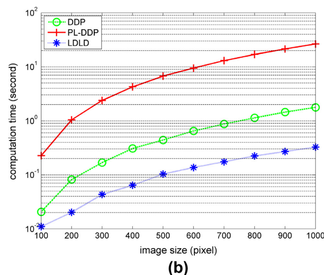
Fig. 12. Efficiency comparison with respect to different parameters and image sizes. (a) Total computation time on clinical images versus l_{max} between PL-DDP and LDLD. (b) Computation time on synthetic images versus image sizes among the three methods.
